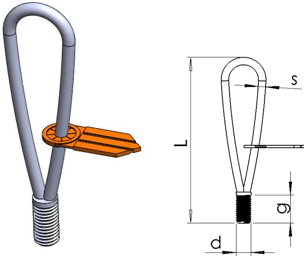
Figure 10 Universal lifter dimension sketch.
