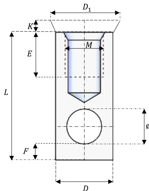
Figure 9 Lifting socket solid material sketch.
