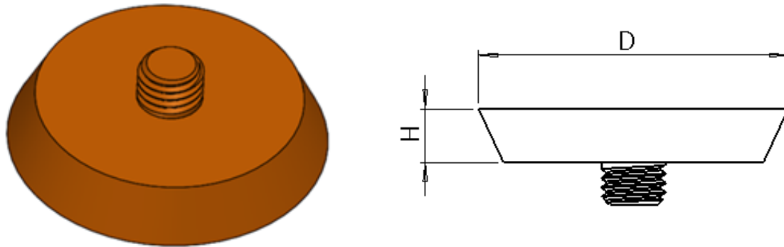
Figure 12 Nailing plates for Lifting socket solid materials.
