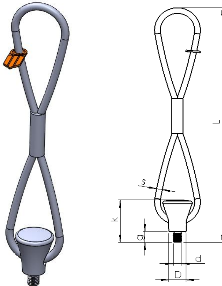
Figure 11 Goliath Lifting loop 40.8-dimension sketch.
