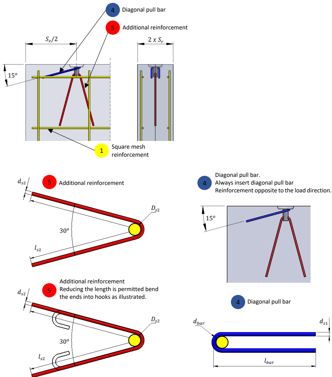
Figure 7 Reinforcement in the concrete wall
