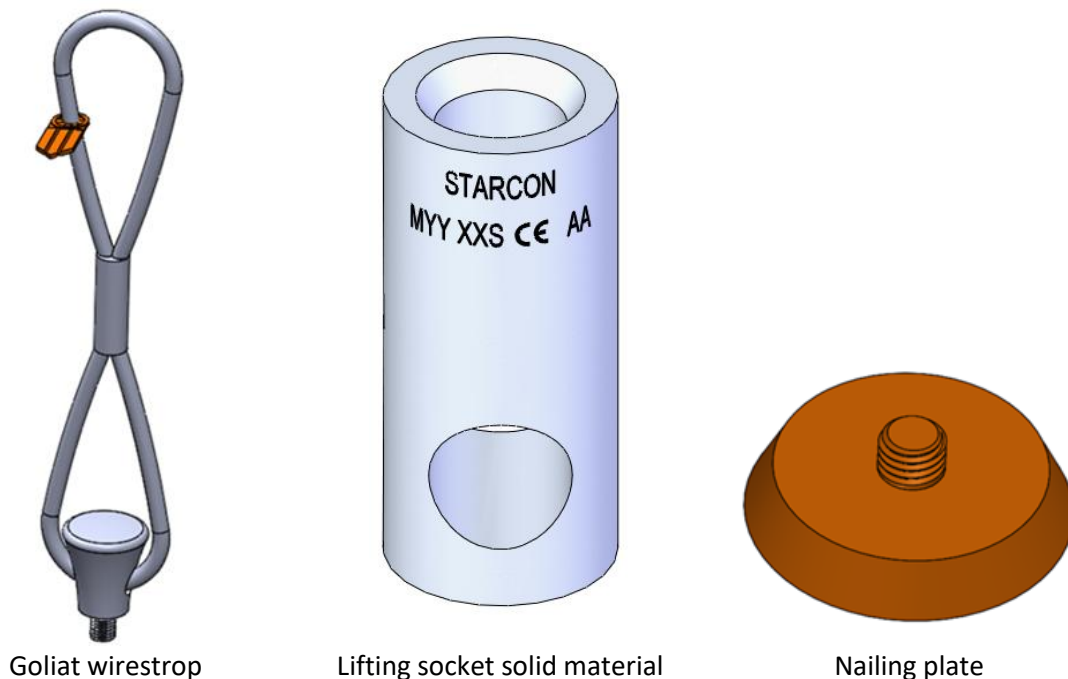
Figure 1 Starcon lifting system.
