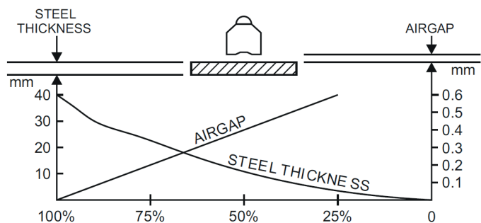
Model POWERTEX 300 kg
