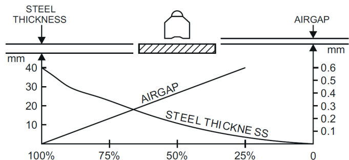
POWERTEX rated output 600 kg
